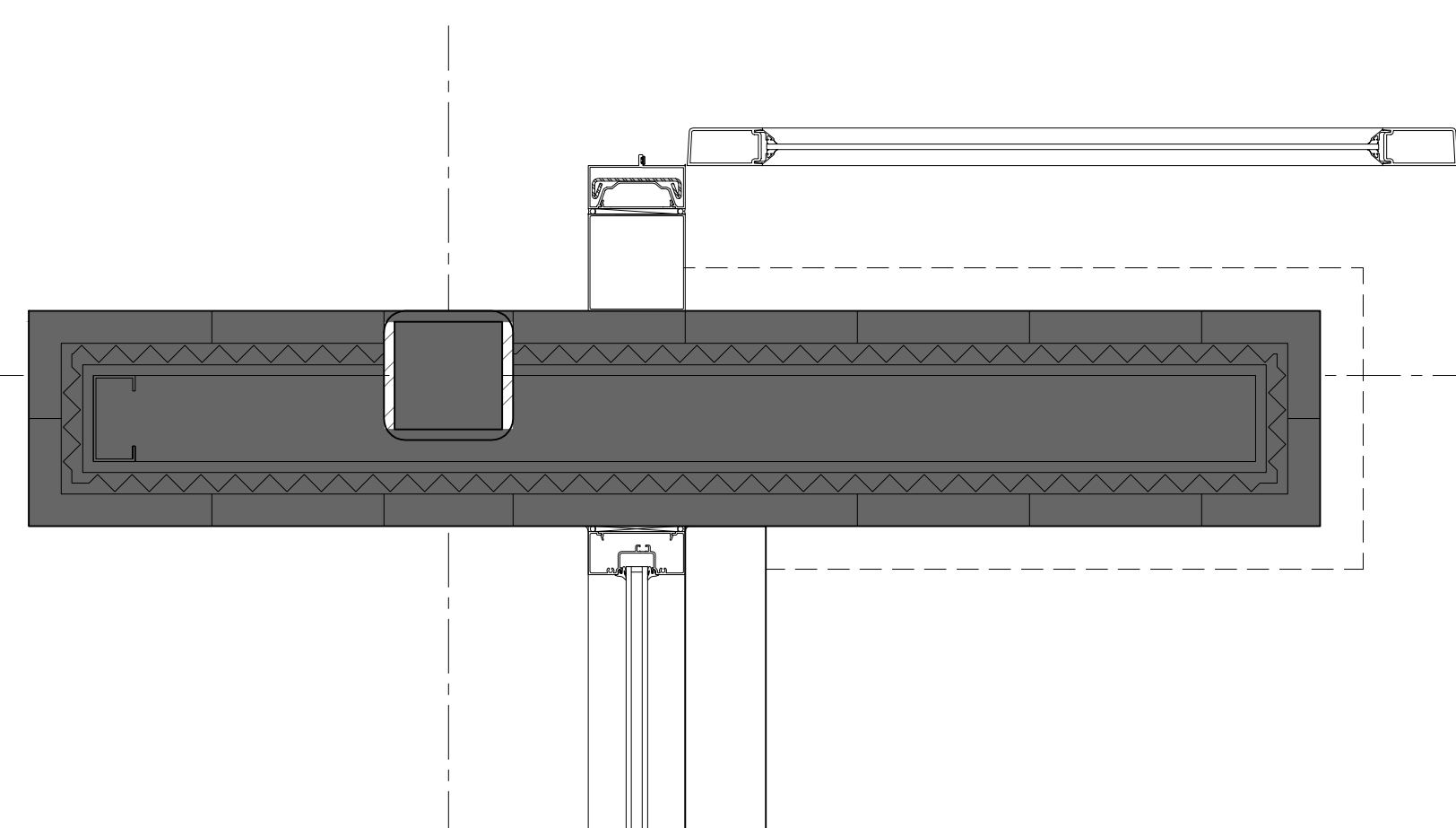
SECTION DETAIL 1 1/2"=1'-0" 15
