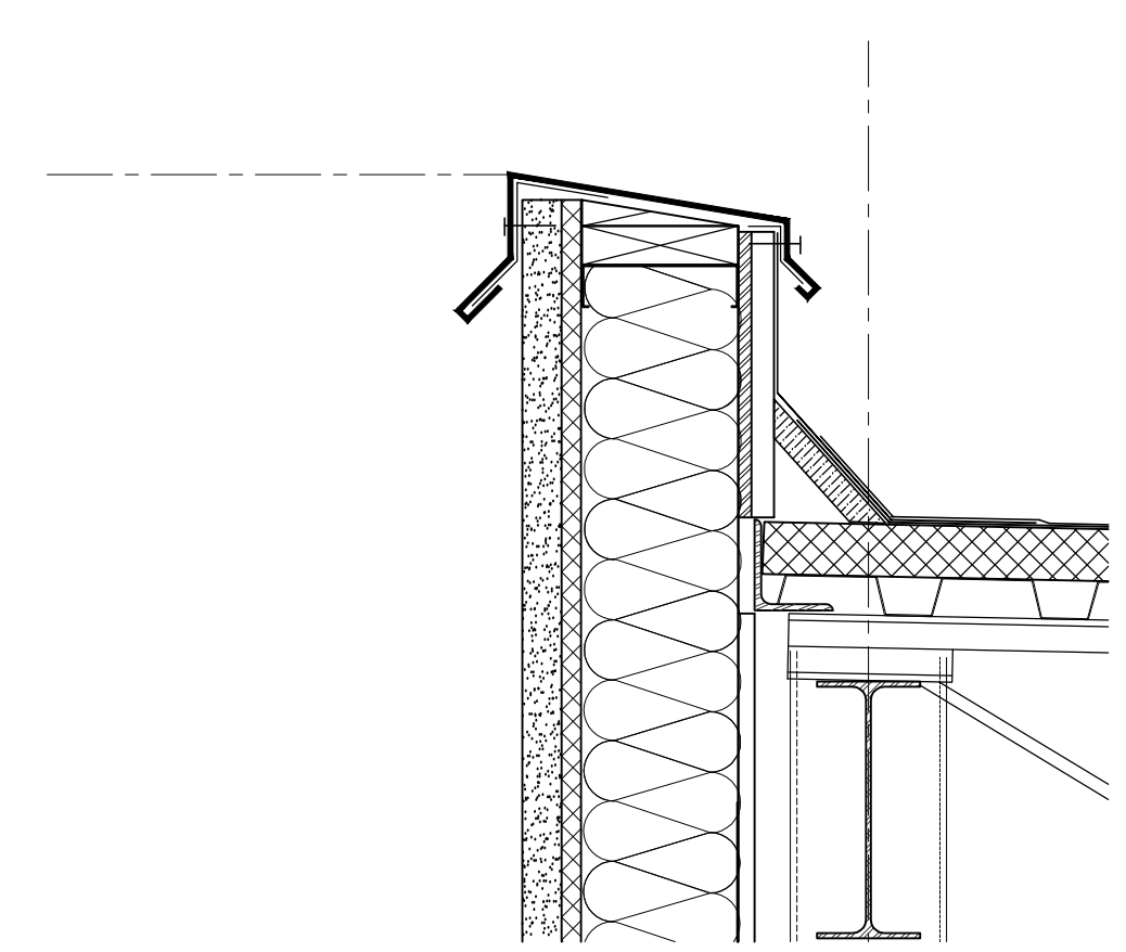
SECTION DETAIL 1 1/2"=1'-0" 8
