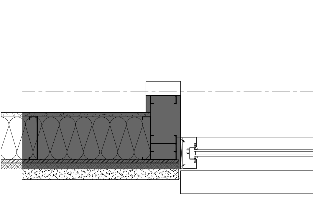
SECTION DETAIL 1 1/2"=1'-0" 20
