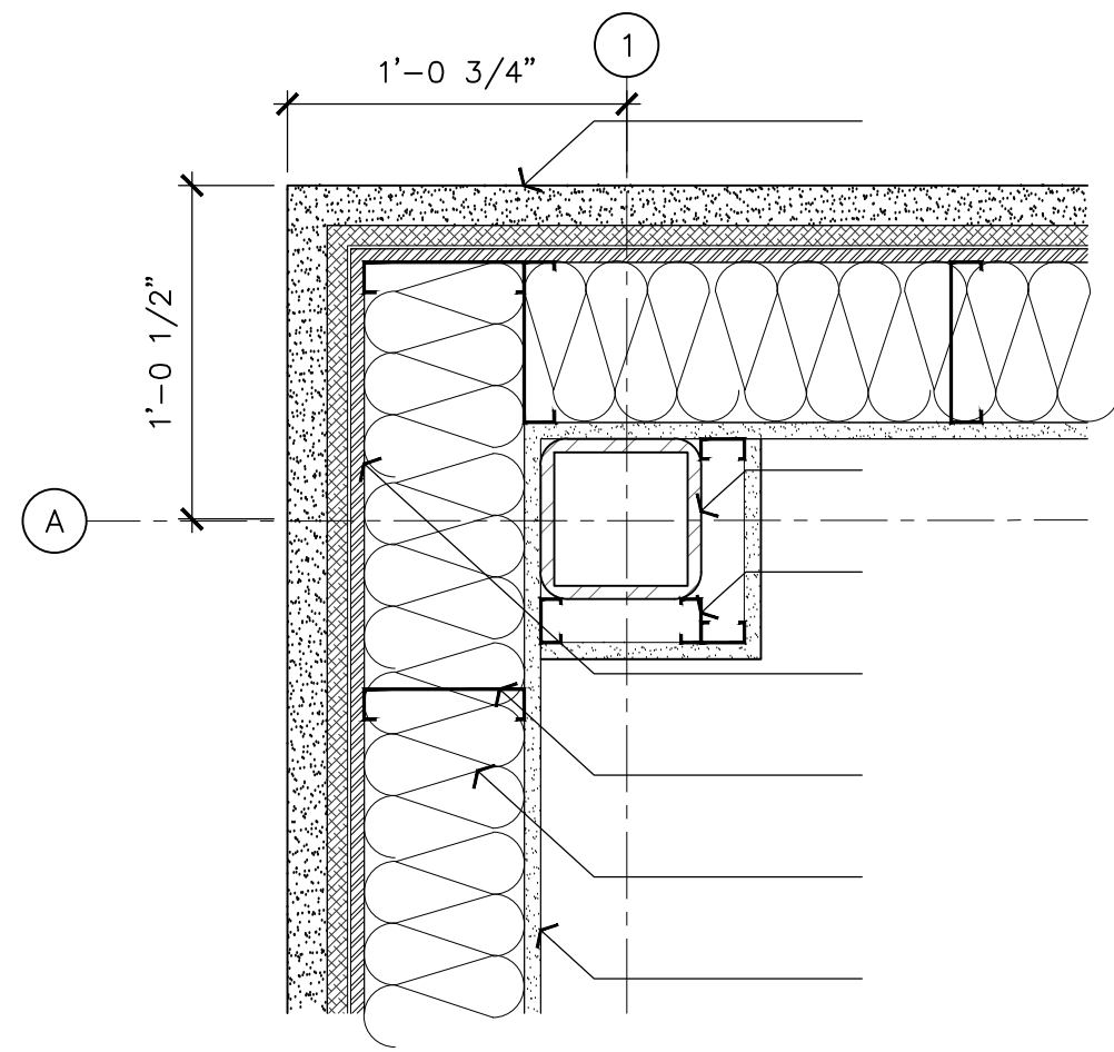
SECTION DETAIL 1 1/2"=1'-0" 20
