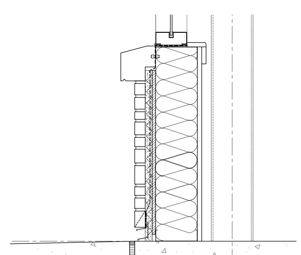
SECTION DETAIL 1 1/2"=1'-0" 2
