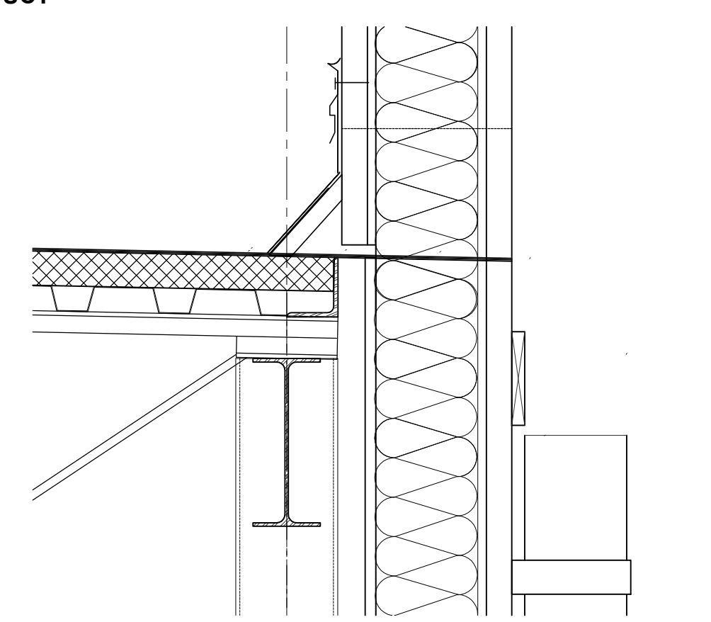
SECTION DETAIL 1 1/2"=1'-0" 12
