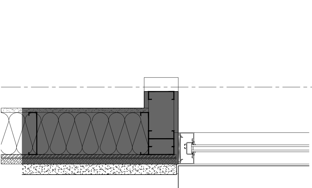
SECTION DETAIL 1 1/2"=1'-0" 19
