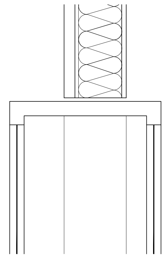
SECTION DETAIL 1 1/2"=1'-0" 10
