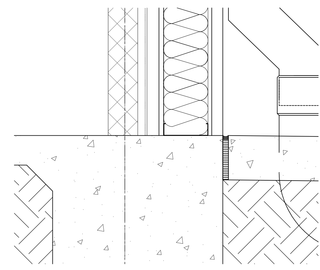
SECTION DETAIL 1 1/2"=1'-0" 7
