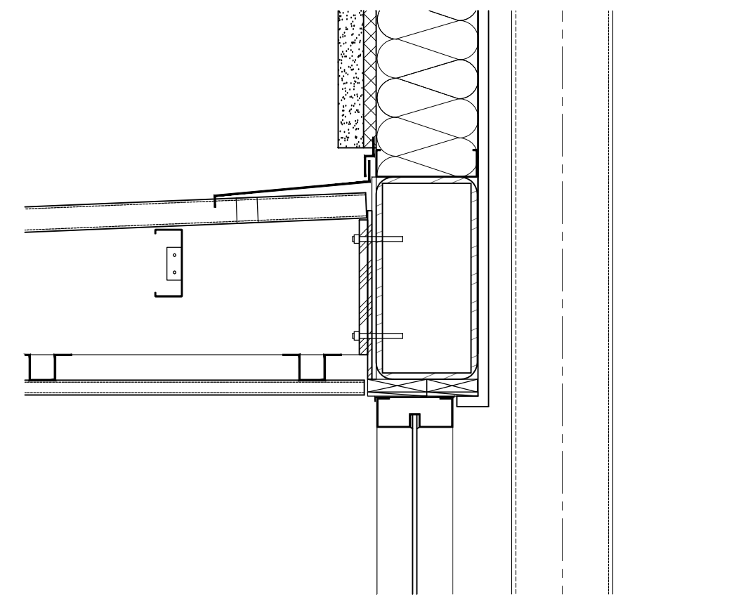
SECTION DETAIL 1 1/2"=1'-0" 2
