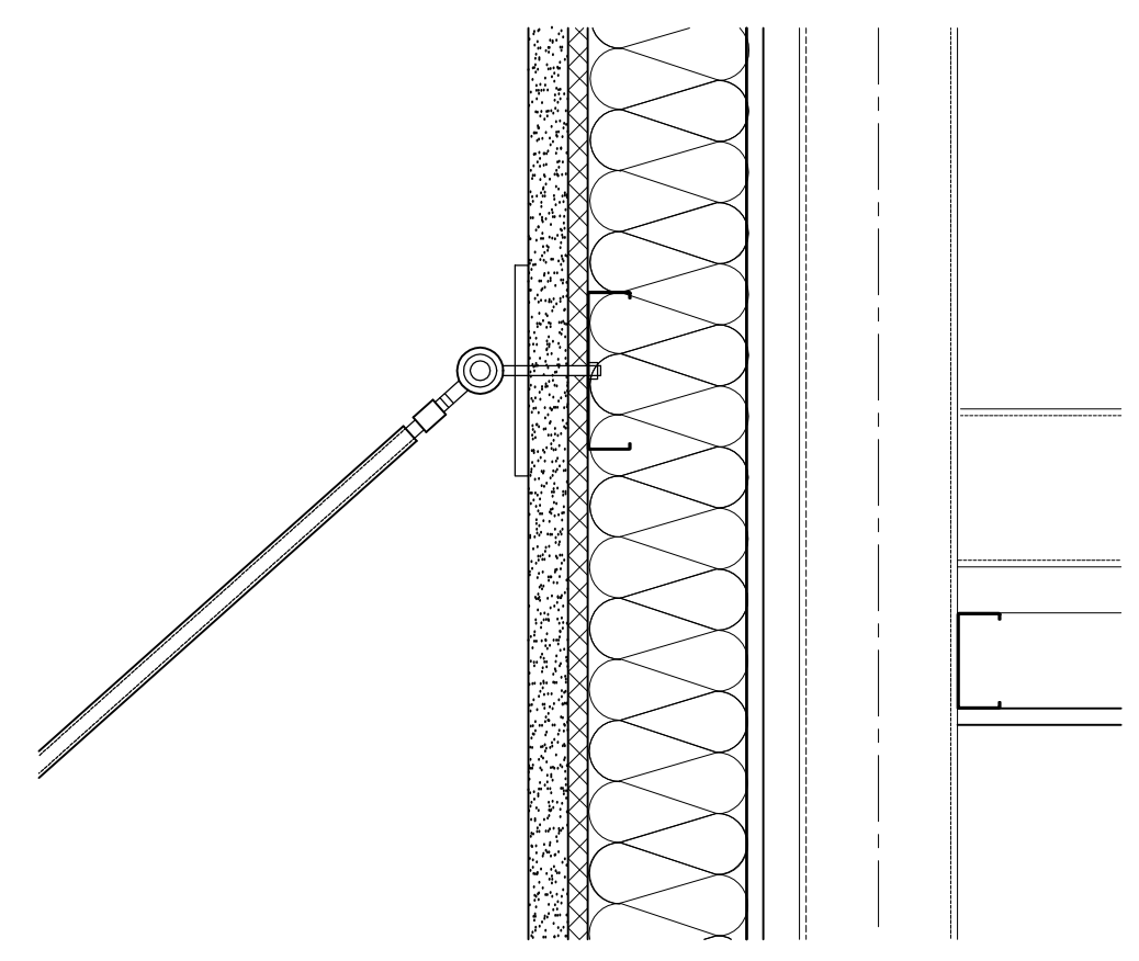
SECTION DETAIL 1 1/2"=1'-0" 3
