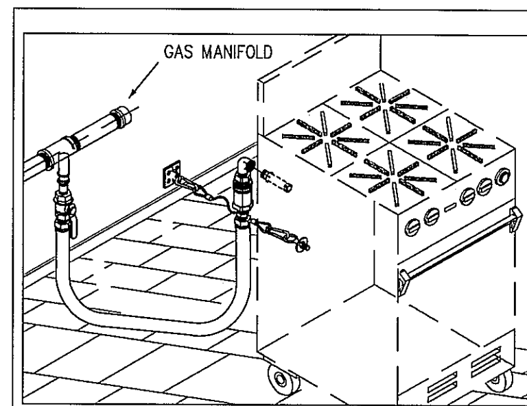
STANDARD GAS QUICK DISCONNECT INSTALLATION
