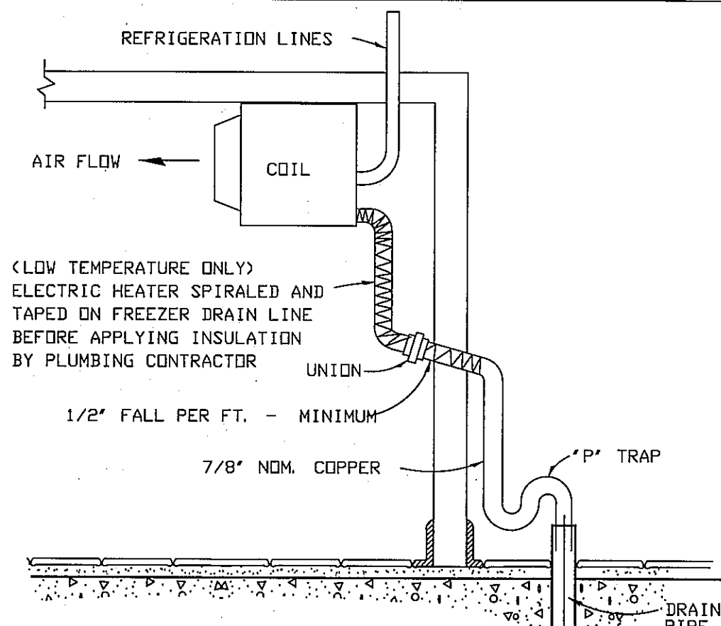
TYPICAL COOLER/FREEZER DRAIN INSTALLATION
