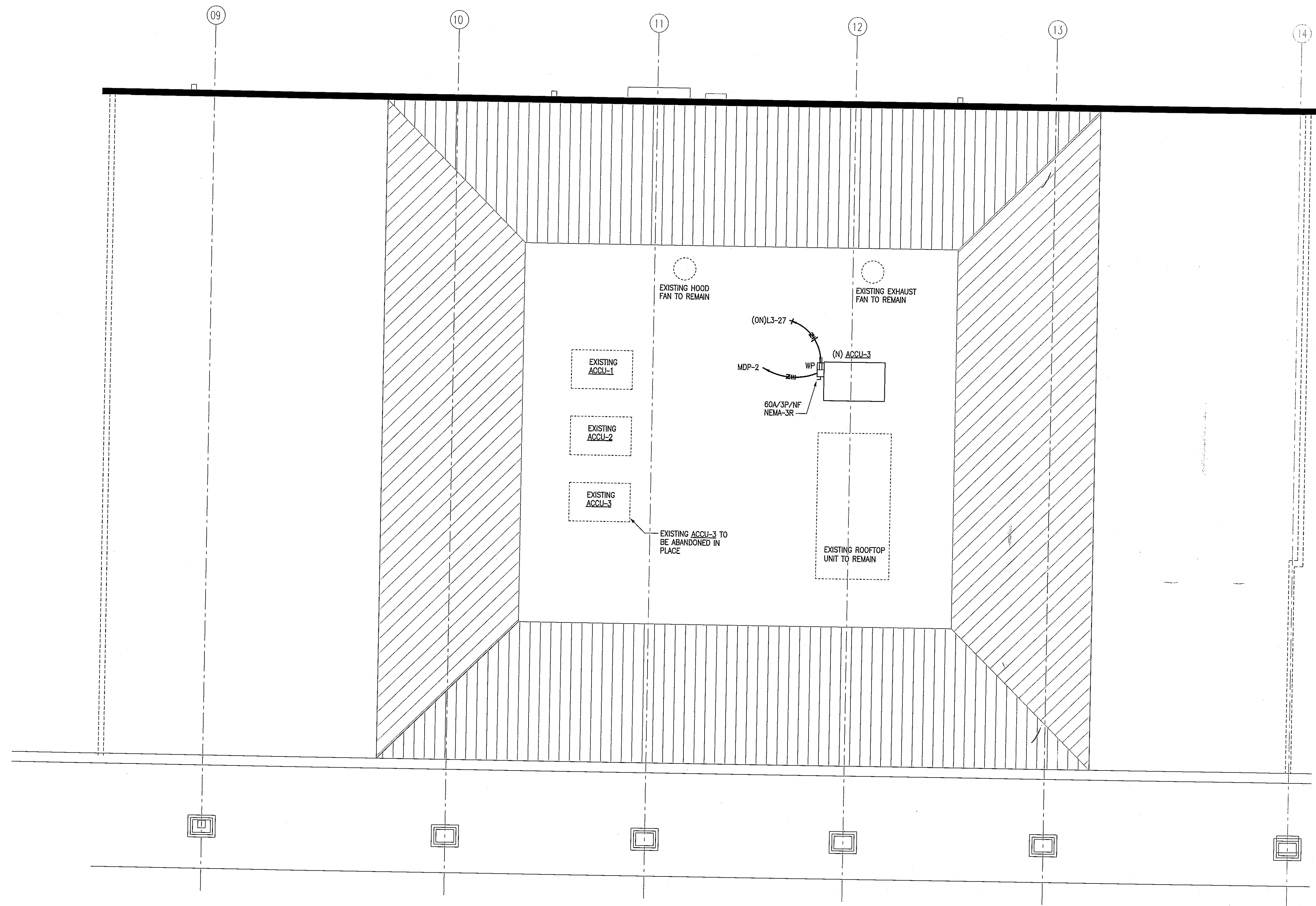
1 ELECTRICAL ROOF PLAN SCALE: 3/16" = 1'-0"
