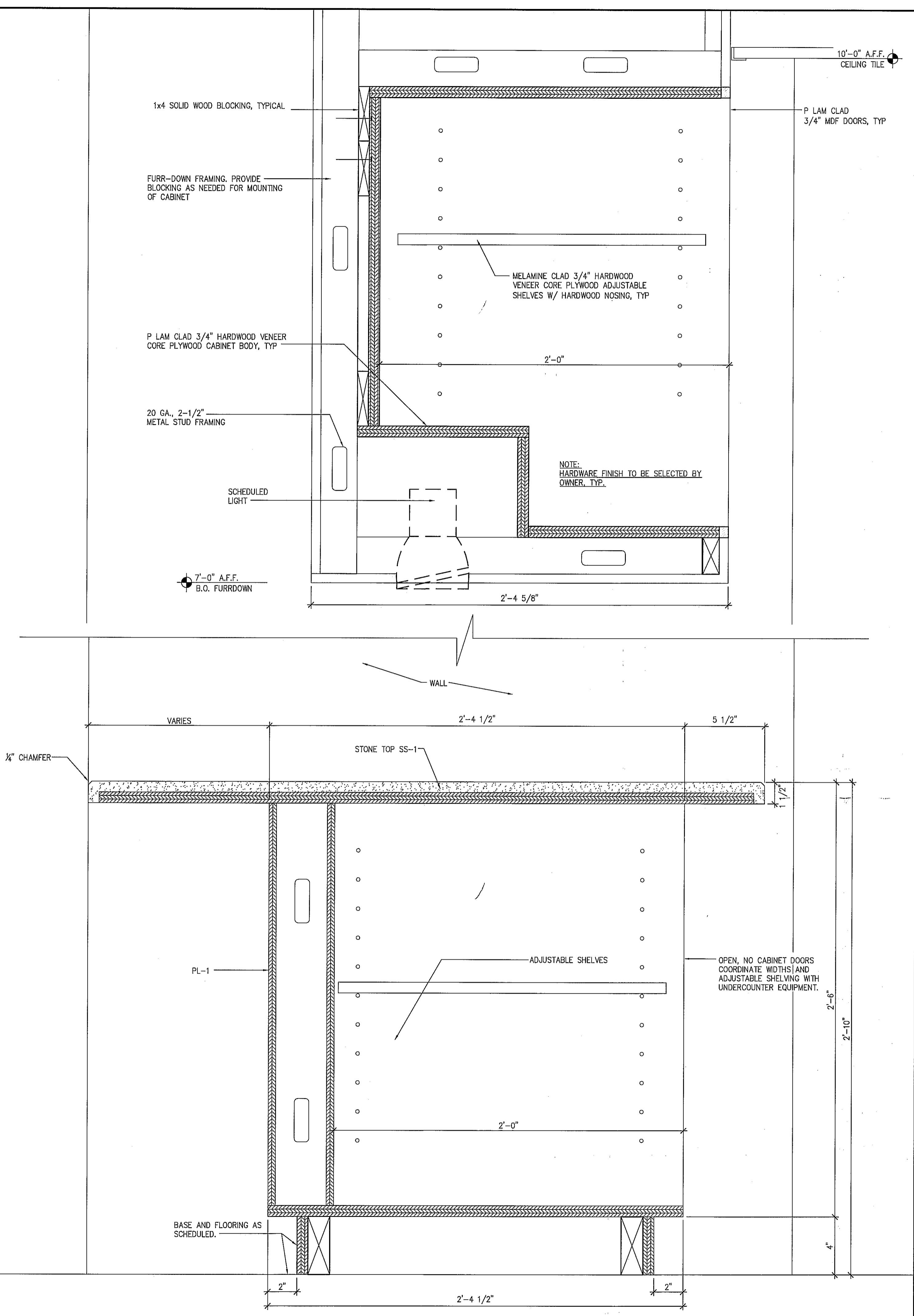
SECTION @ PICK-UP
