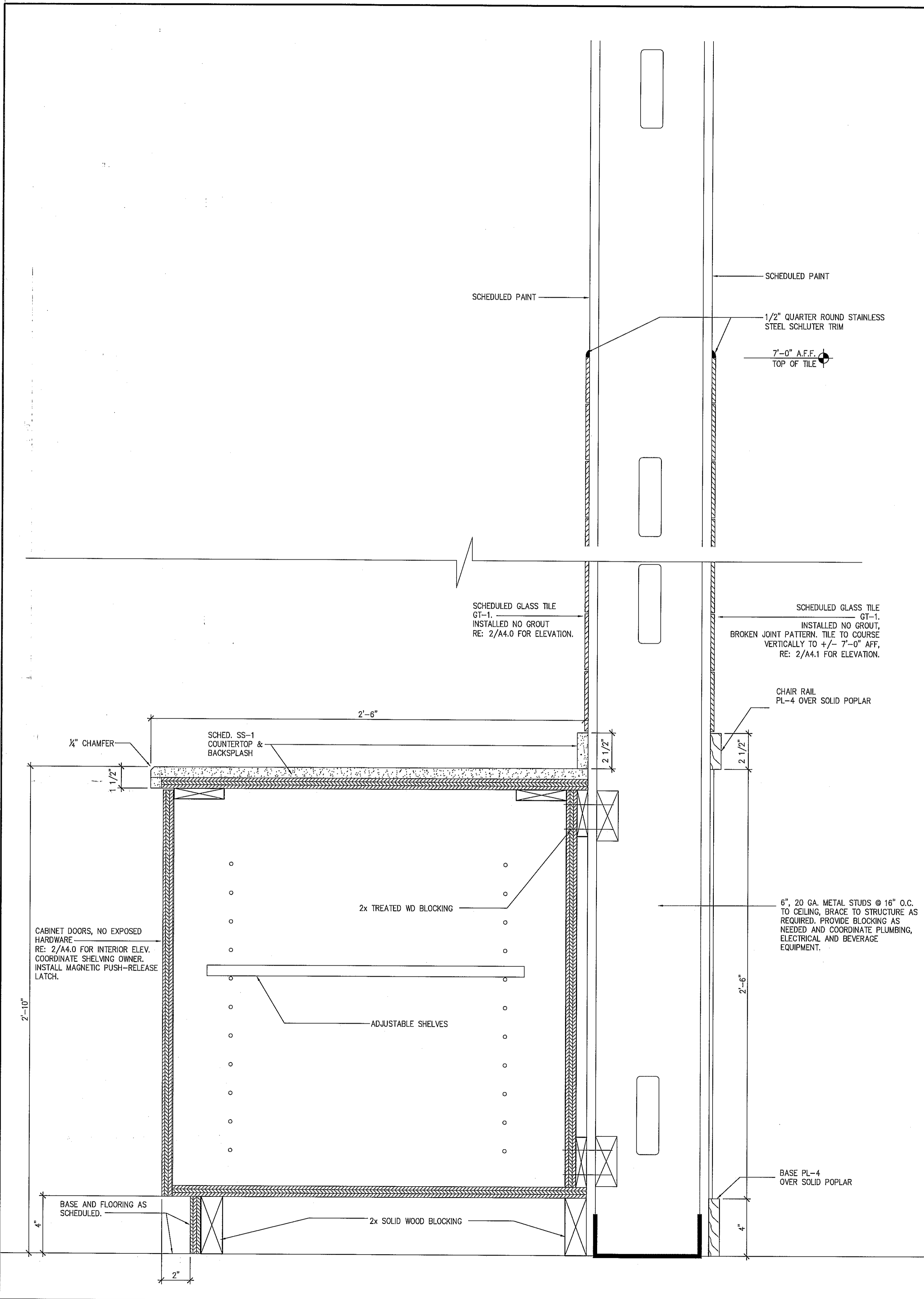
SECTION @ OASIS COUNTER
