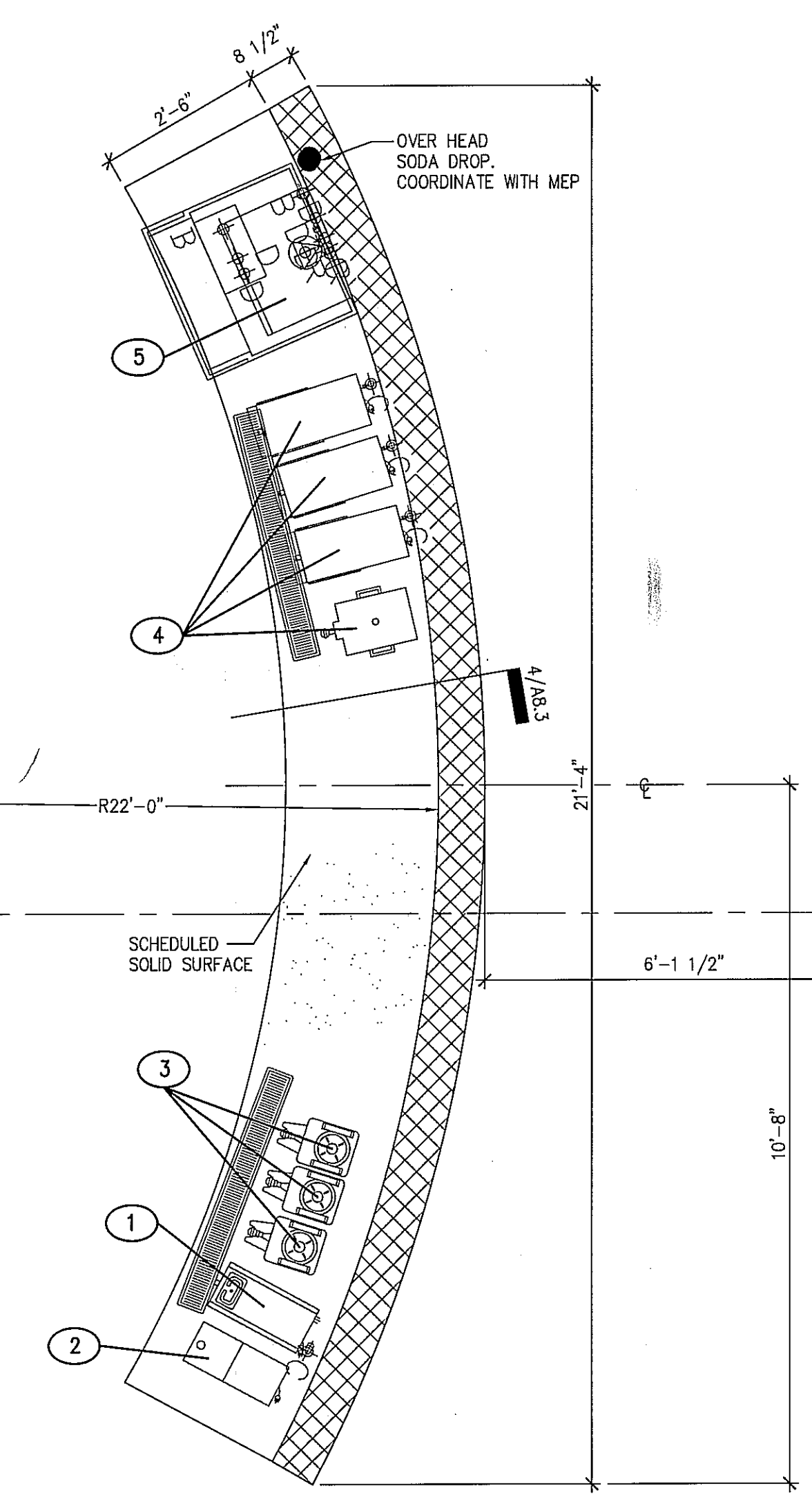
ENLARGED FLOOR PLAN- BEVERAGE COUNTER
