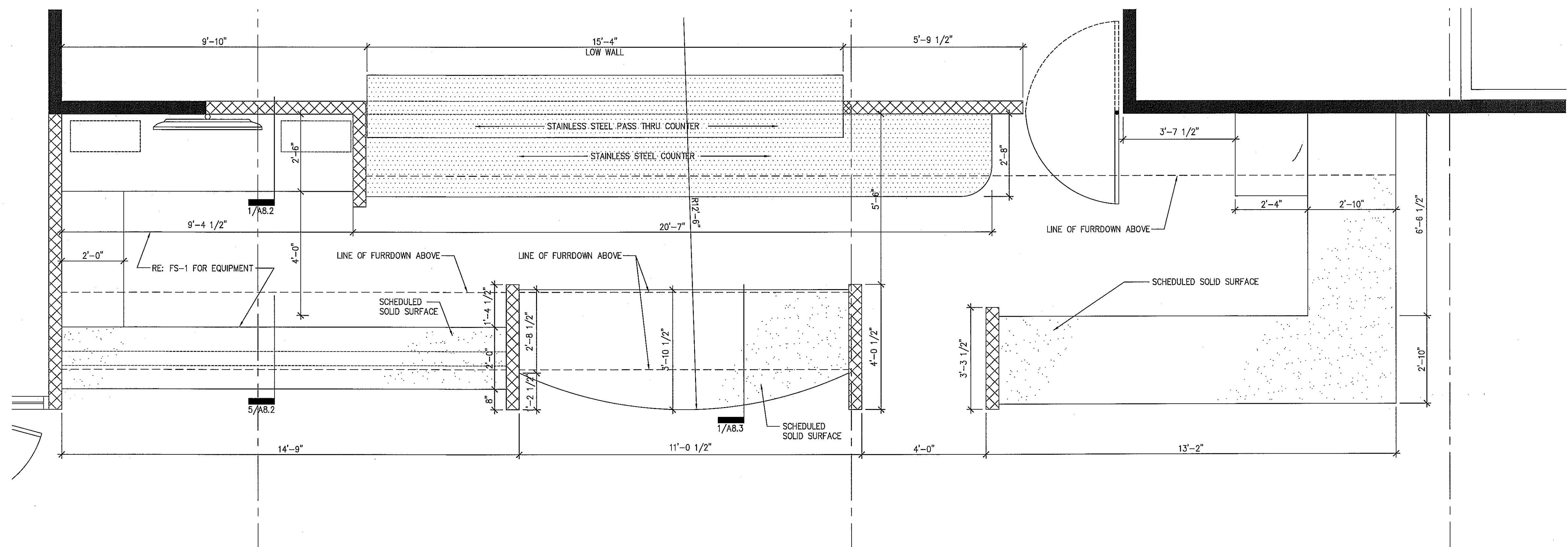
ENLARGED FLOOR PLAN- BEVERAGE COUNTER
