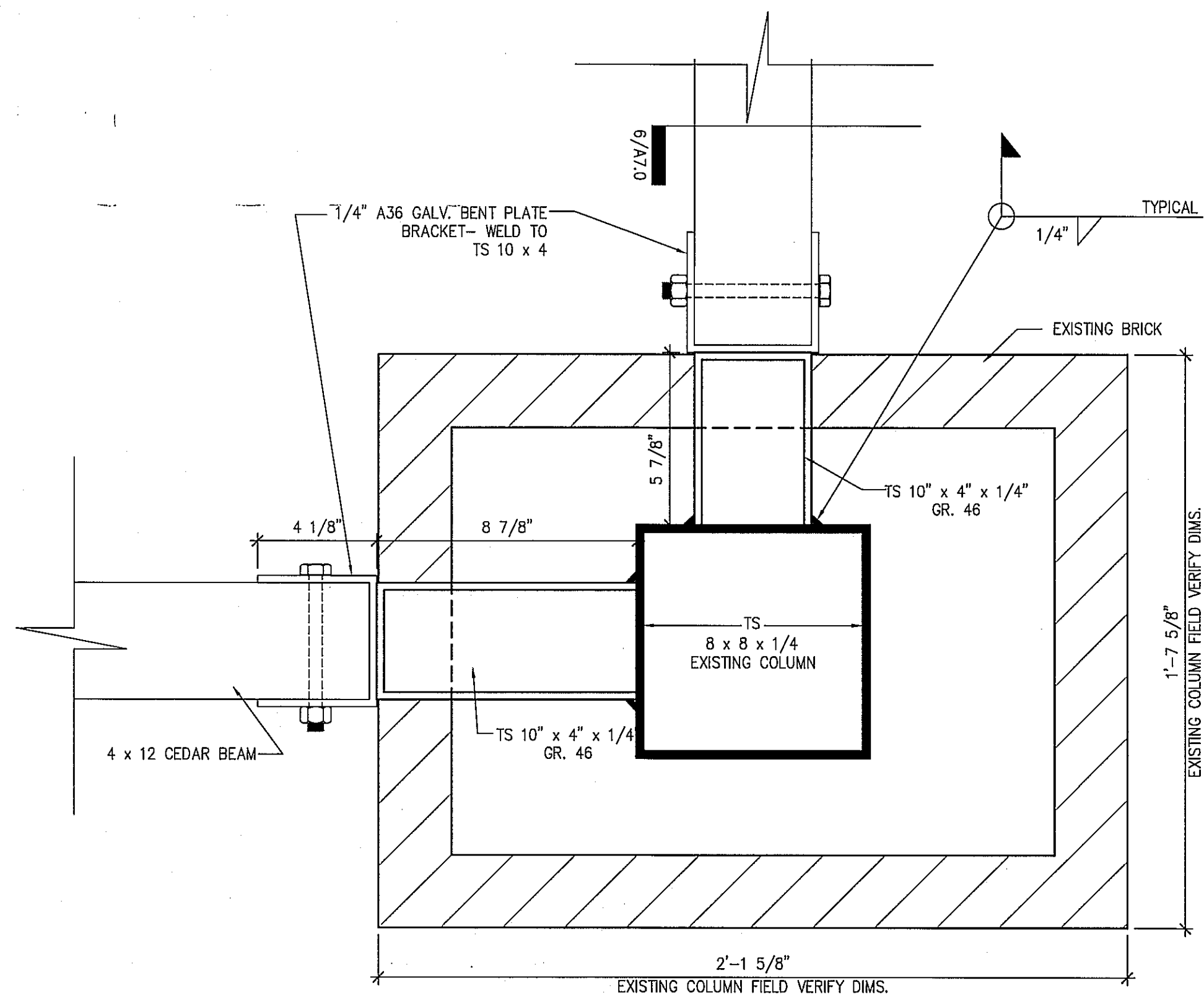
SECTION -BEAM CONNECTION
