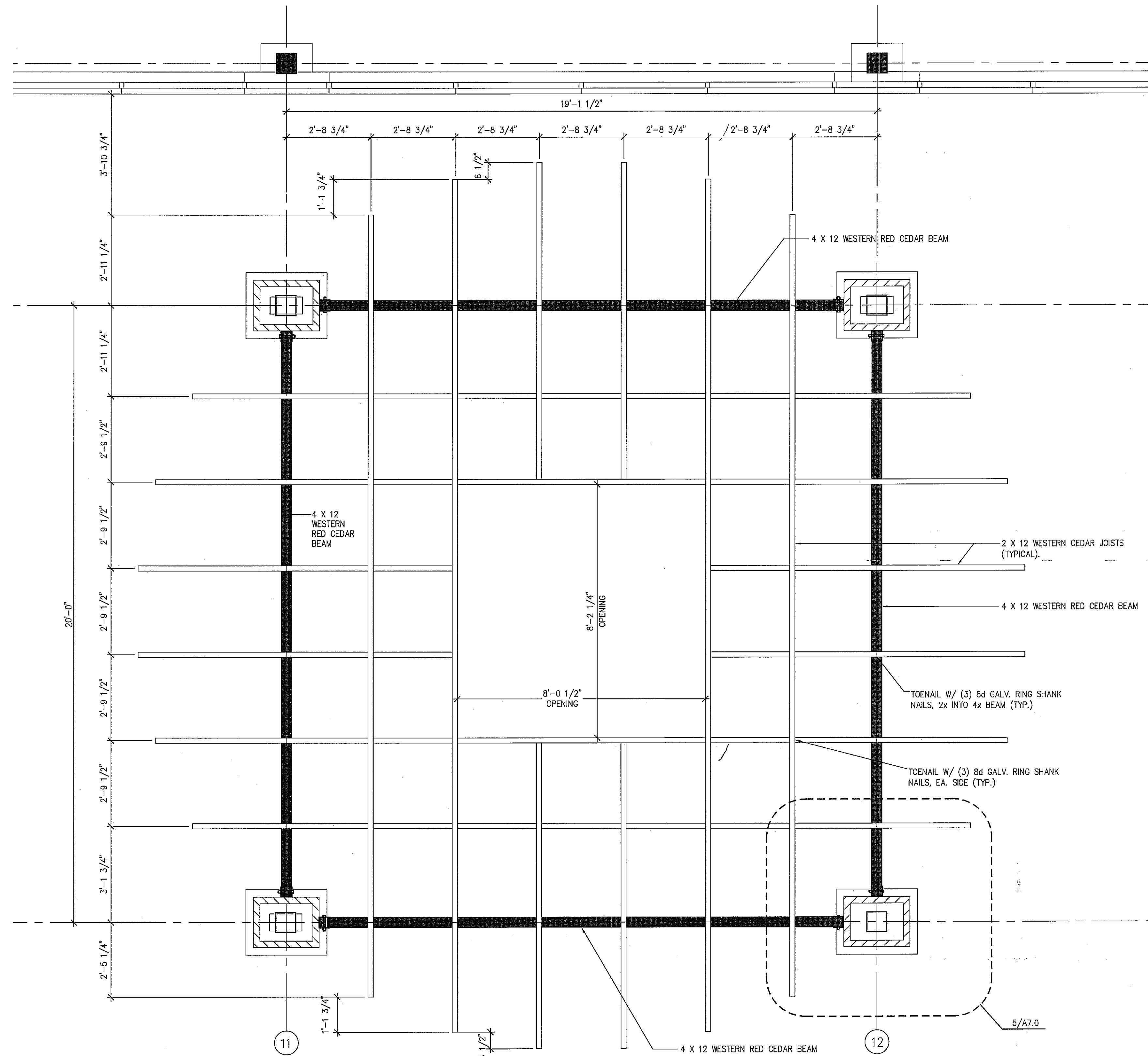
ENLARGED PERGOLA PLAN
