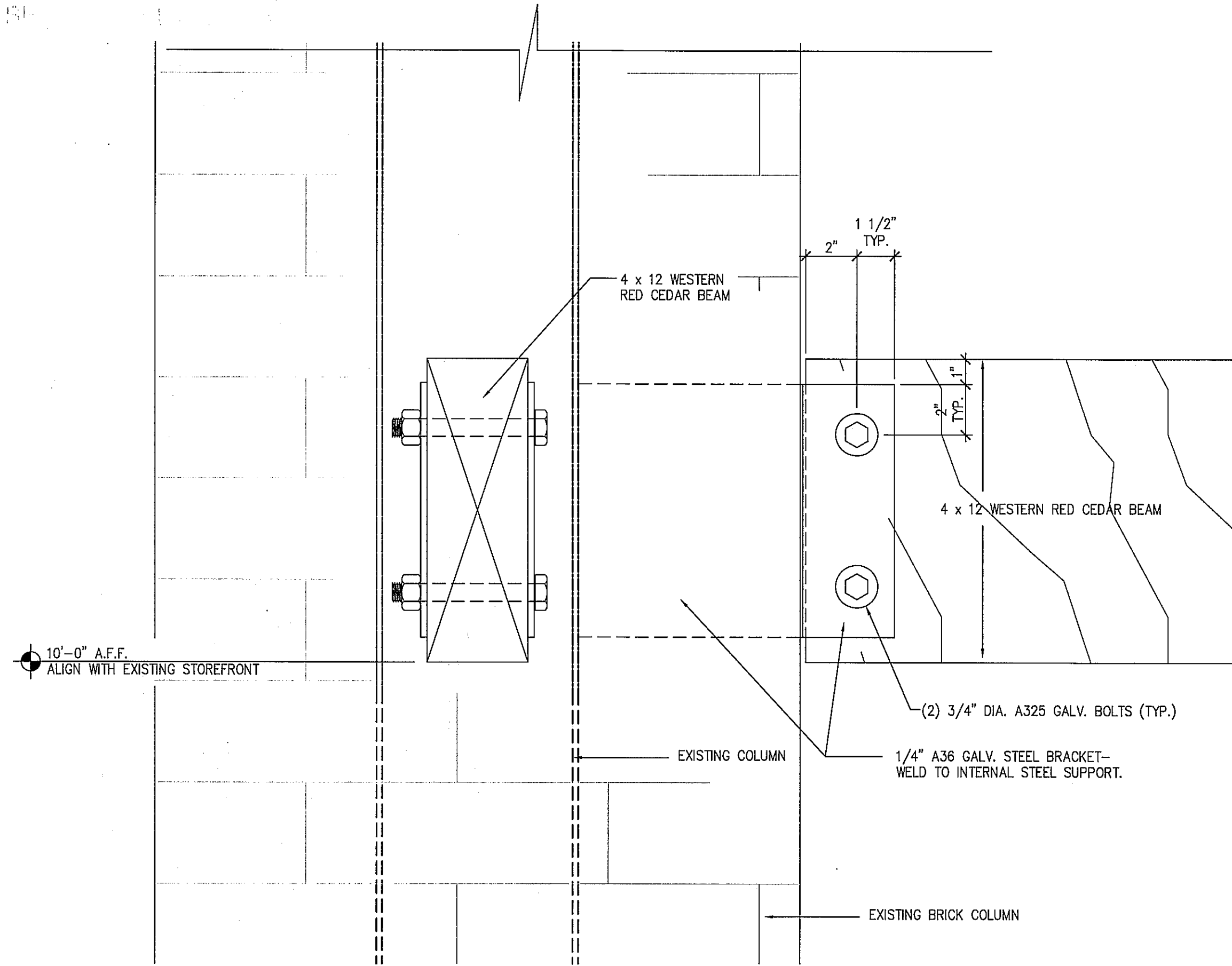
SECTION -BEAM CONNECTION
